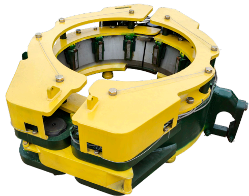
36-inch 125-ton JET STRING ELEVATOR™
