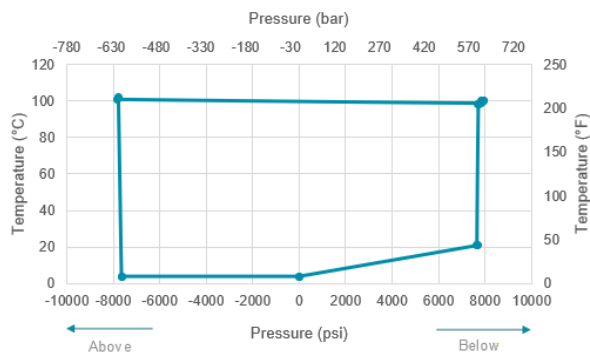
Rated Performance Envelope
