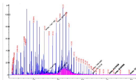
GC C36 plot WFS sample with 30% mud contamination
